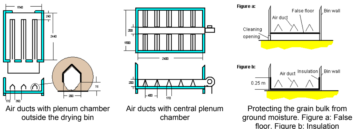
Figure 23: Examples for air duct configurations in fixed bed batch dryers for low-temperature drying
