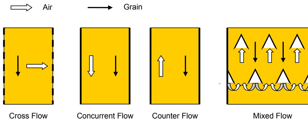
Figure 20: Air flow relative to grain flow in the drying section of continuous dryers
