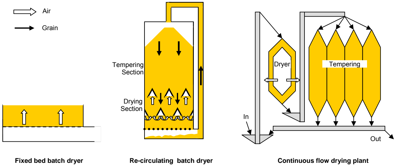
Figure 12: Dryer classification according to crop holding / crop flow
