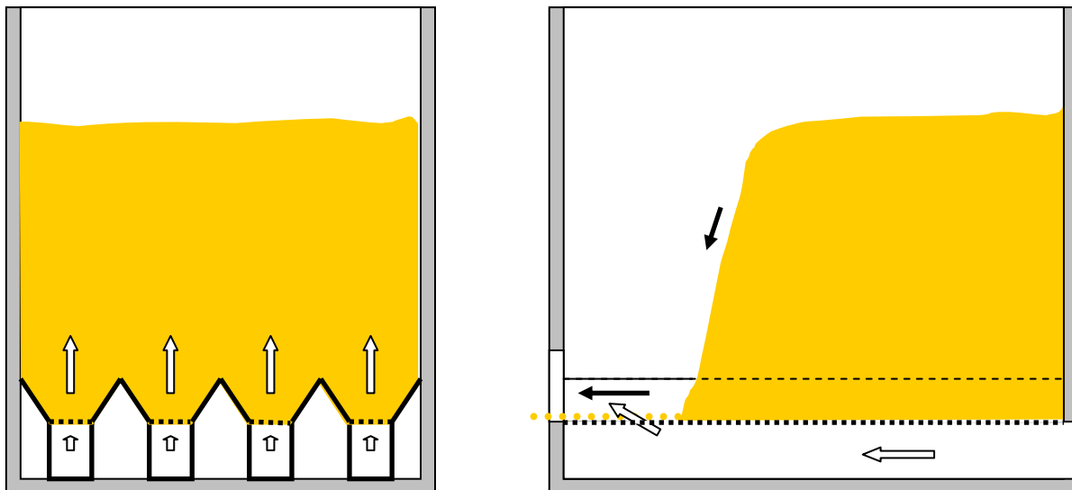
Figure 25: Cross section of a drying bin with 4 air-sweep channels (left) and through one channel while unloading (right)
