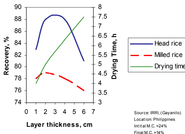
Figure 10: Effect of layer thickness during sun drying on head rice recovery, milled rice recovery and drying time.
