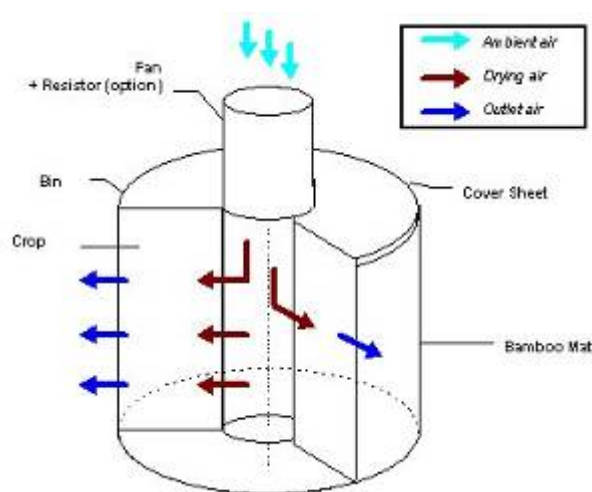
Figure 15: Vietnamese low-cost dryer with circular drying bin made from locally available materials,
