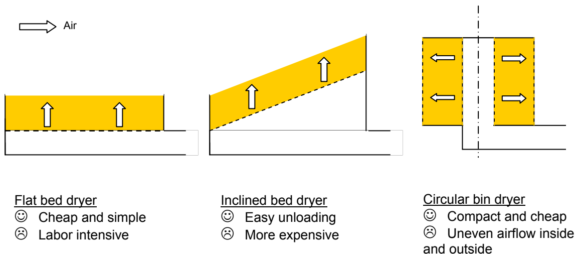
Figure 13: Bed configuration of fixed bed batch dryers
