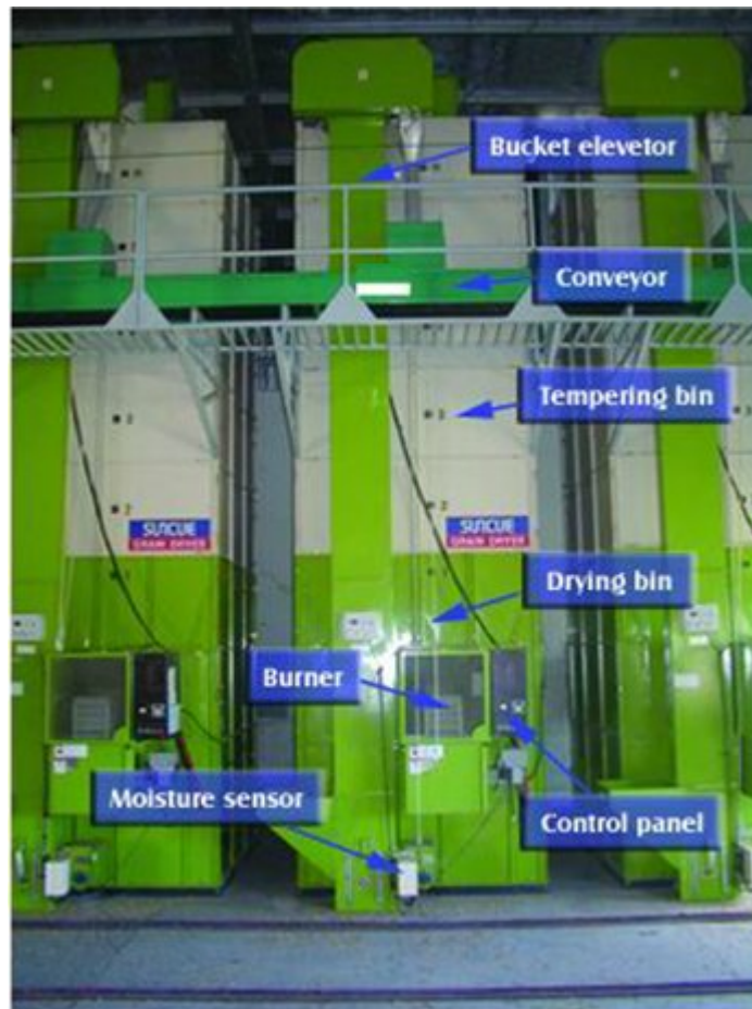
Figure 18: Components of a re-circulating batch dryer
