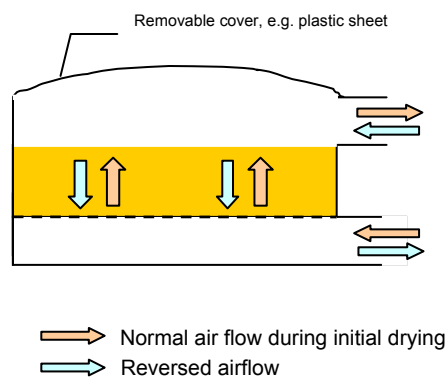
Figure 16: Principle (left) and example of a mobile reversible-flow batch dryer (right)
