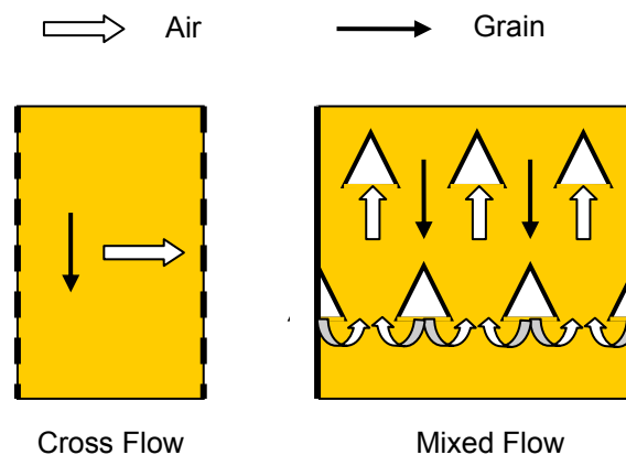
Figure 19: Air flow relative to grain flow in the drying section of re-circulating batch dryers
