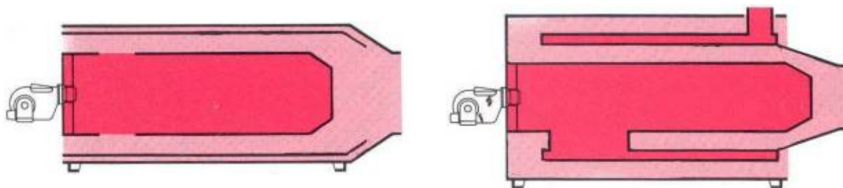
Figure 28: Direct fired (left) and indirect fired (right) air heaters, both with kerosene burner
