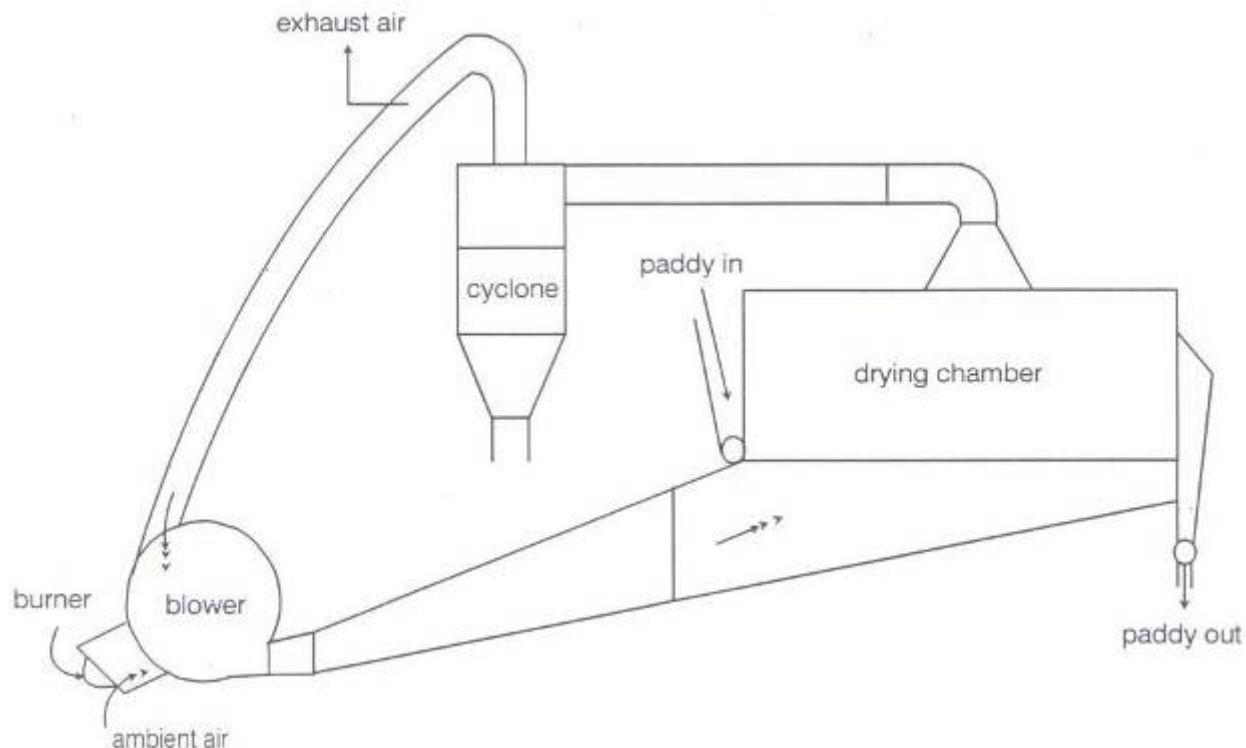
Figure 21: Principle of a Thai fluidized bed dryer for first-stage drying down to 18% MC (Soponronnarit, 1996)
