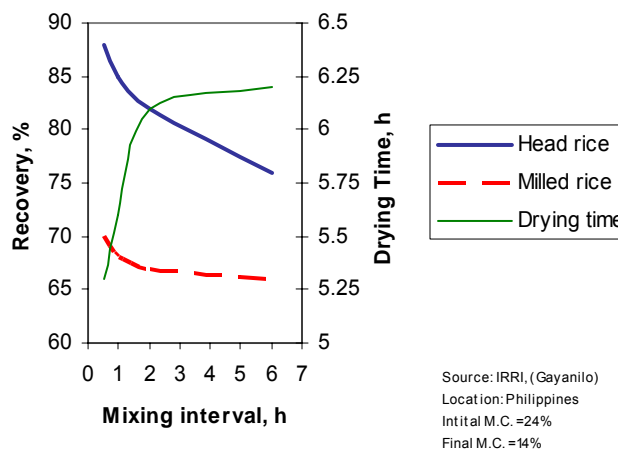
Figure 11: Effect of the mixing interval during sun drying on head rice recovery, milling recovery and drying time
